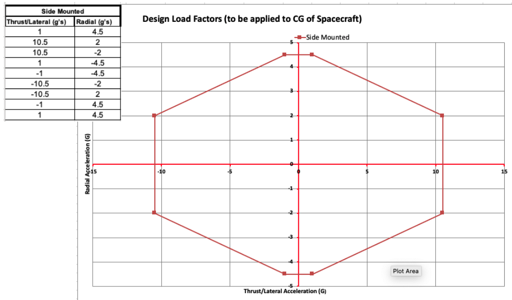
Figure 6.2 Side Mounted Design Load Factors (Updated in Rev 2)
